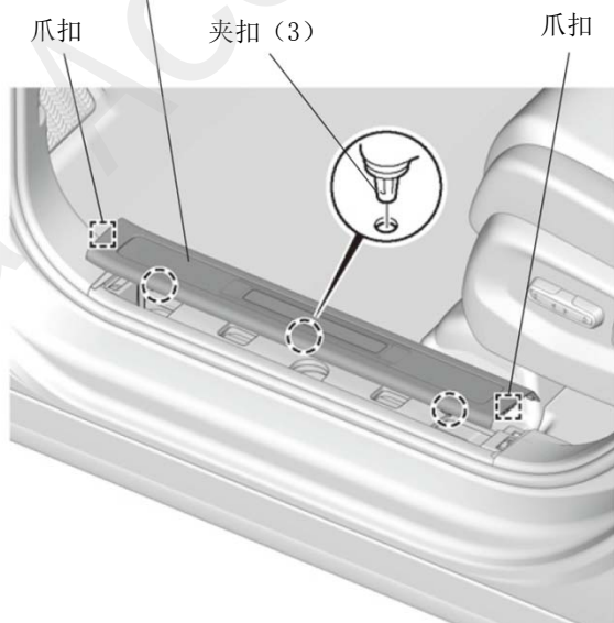
左前 LED 迎宾踏板
